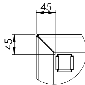
DETAIL I SCALE 1 : 5
