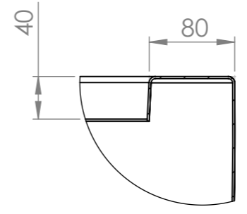
DETAIL 1 SCALE 1 : 5
