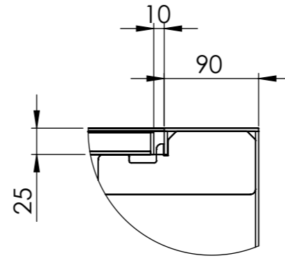
DETAIL D SCALE 1 : 5
