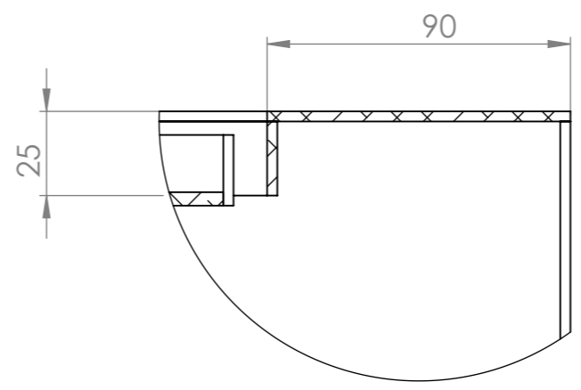
DETAIL E SCALE 1 : 2
