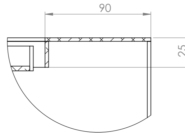
DETAIL E SCALE 1 : 2
